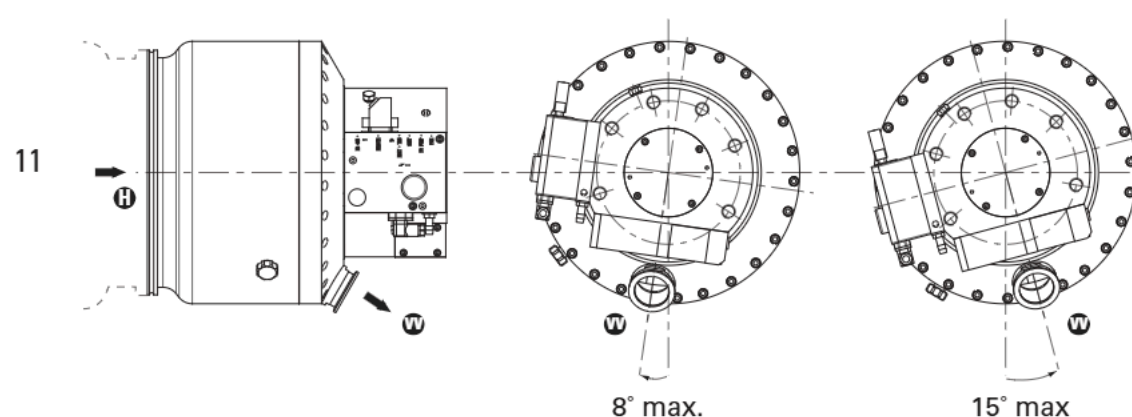
Horizontal installation position of the turbopump
