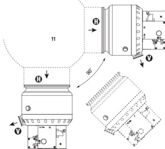
Permissible installation positions for the turbopump
