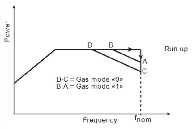
Gas type characteristic line
