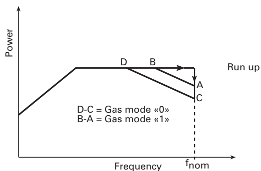
Gas type characteristic line
