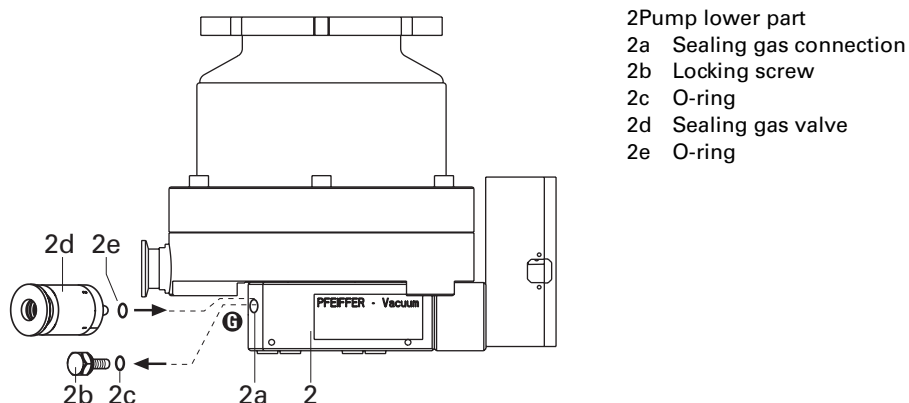
Fig. 6: Connecting the sealing gas valve
