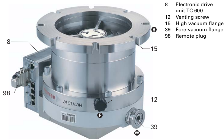
Fig. 2: View of CompactTurbo™ TMH 521 P
