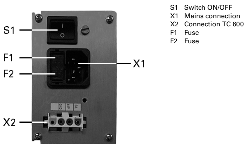
Fig. 9: Rear panel of power supply TPS
