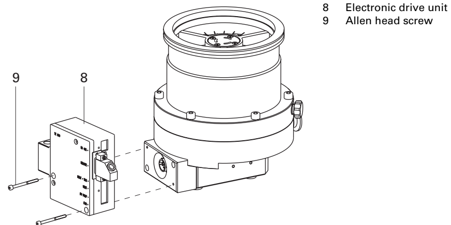
Fig. 11: Assembly / disassembly of the TC 600
