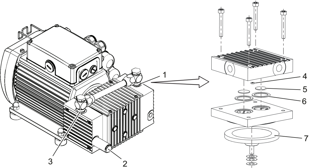
Fig. 6: Spare parts
