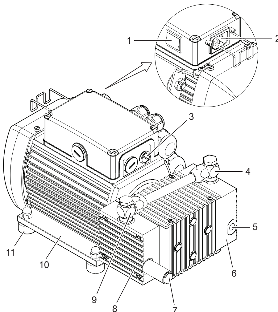
Fig. 2: Diaphragm pump design
