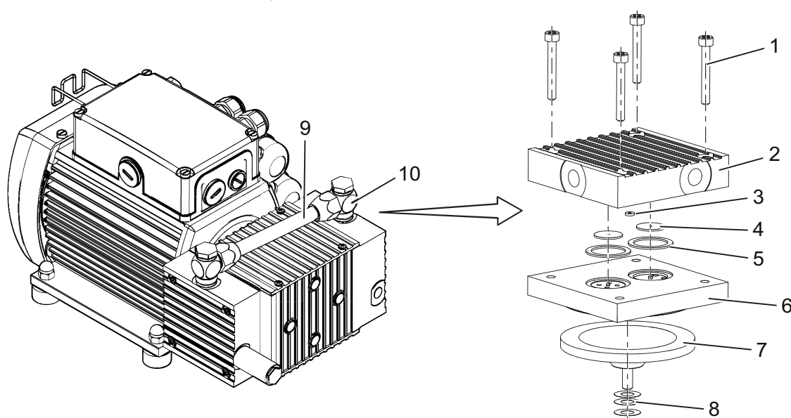
Fig. 4: Diaphragm head and valves
