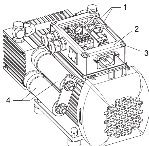
Fig. 5: Device fuses
