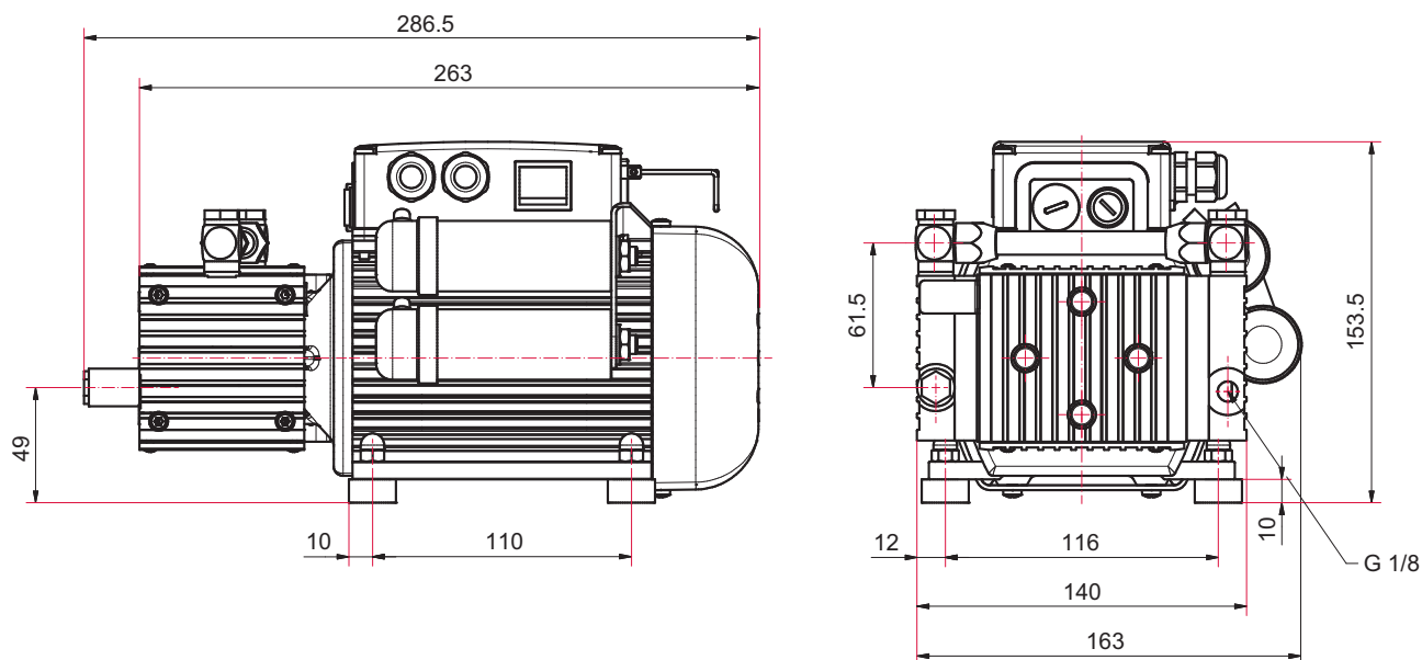
Fig. 7: Dimensions MVP 015-2
